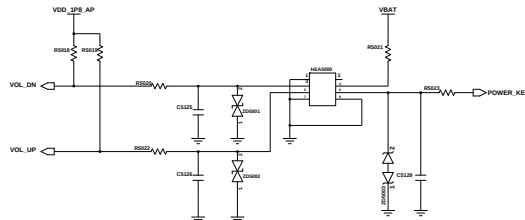
VOLUME KEY POWER KEY
